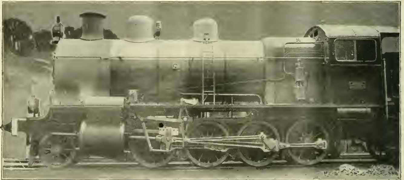
A NORWEGIAN CONSOLIDATION ENGINE.
